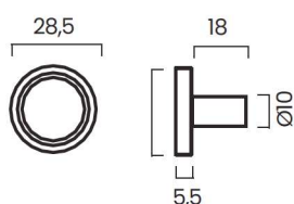
CHISEL knob
