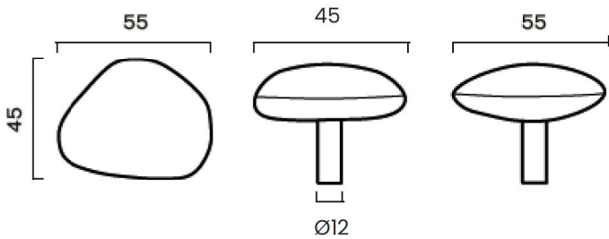
NOBLE knob & hook large
