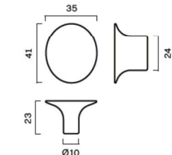
LEAF knob
