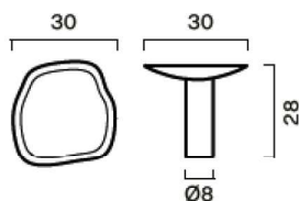
VALE knob
