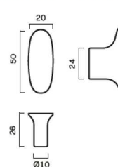
LEAF hook (front mounted / wall)
