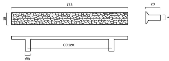
CARVE pull bar
