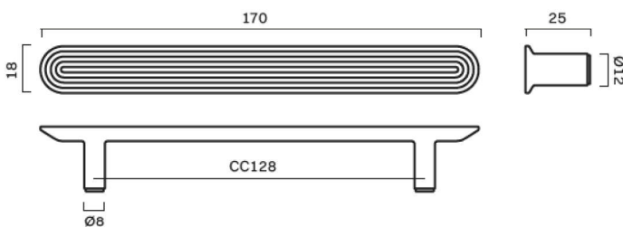
TERRACE pull bar 170 mm
