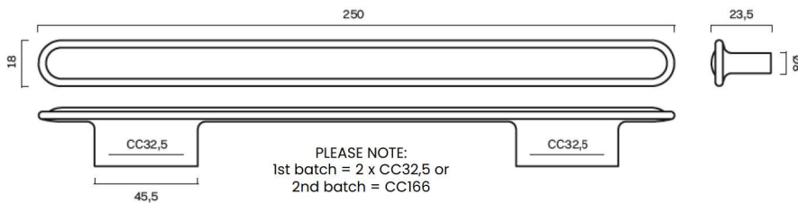
BUTTON pull bar 250 mm
