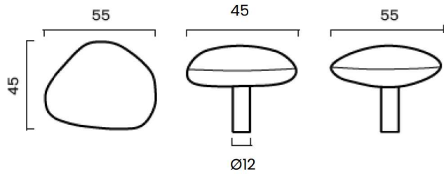
NOBLE knob & hook large
