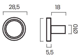
CHISEL knob
