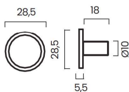
SIGNATURE knob
