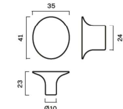
LEAF knob
