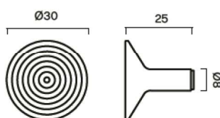
TERRACE knob
