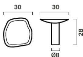
VALE knob
