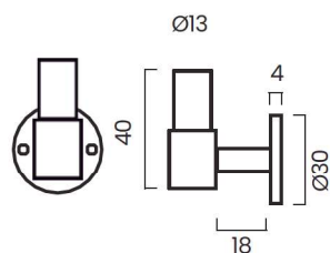
SIGNATURE hook
