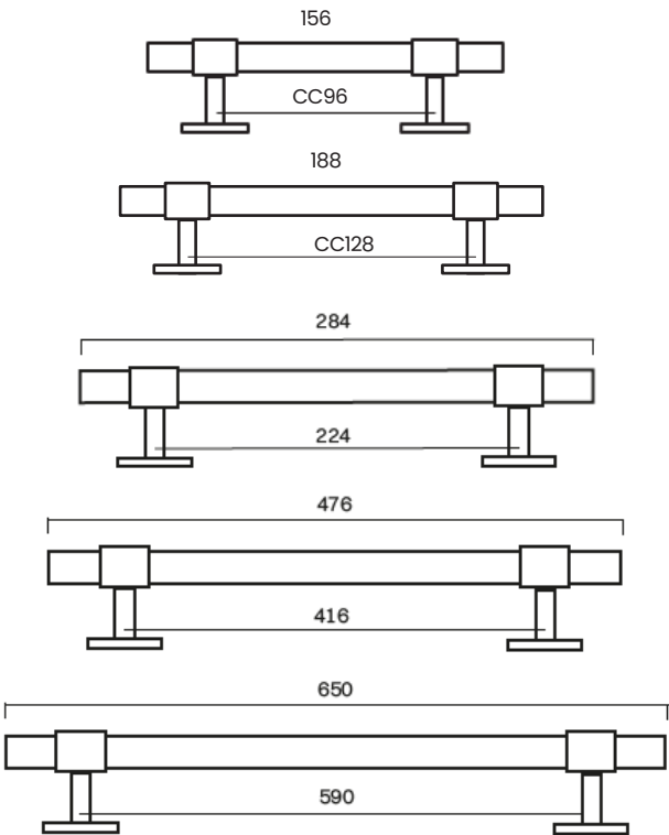
SIGNATURE 30 pull bars
