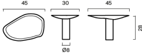
VALE knob oval
