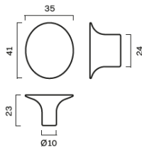
LEAF hook round
