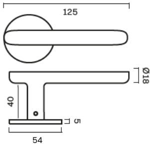
LEAF door handle
