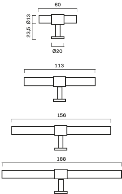
SIGNATURE 20 T-bars
