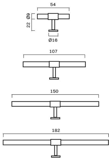
SIGNATURE slim T-bars
