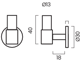
SIGNATURE 30 END knob
