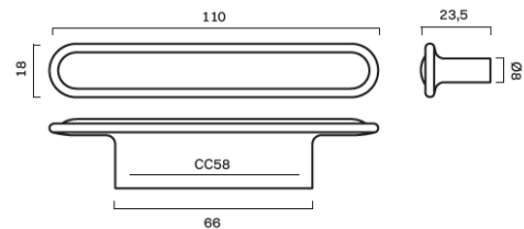
BUTTON pull bar 110 mm
