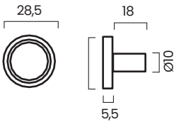
CHISEL knob
