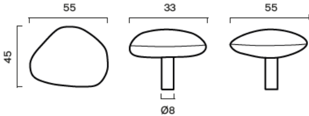
NOBLE knob & hook large
