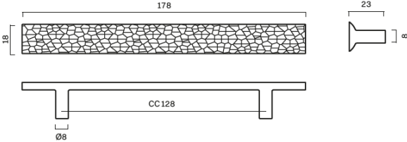
CARVE pull bar
