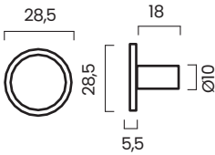
SIGNATURE knob
