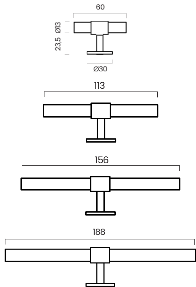
SIGNATURE 30 T-bars
