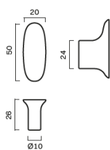
LEAF hook
