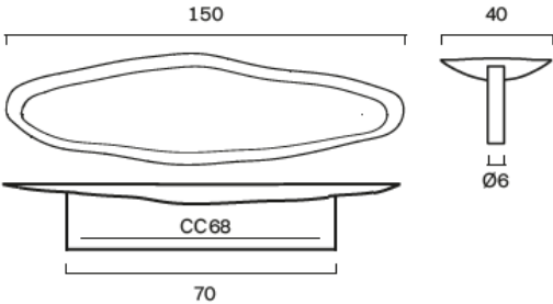
VALE pull bar short
