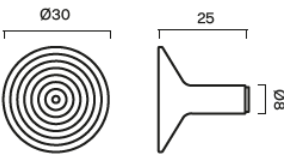
TERRACE knob
