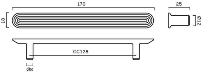
TERRACE pull bar 300 mm
