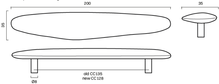
NOBLE pull bar long
